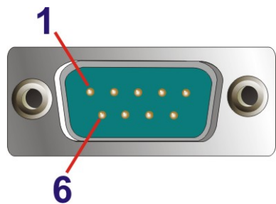
Figure 3-23: RS-232 Connector (COM1, COM2)
