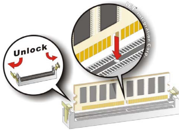
Figure 3-11: DIMM Installation
