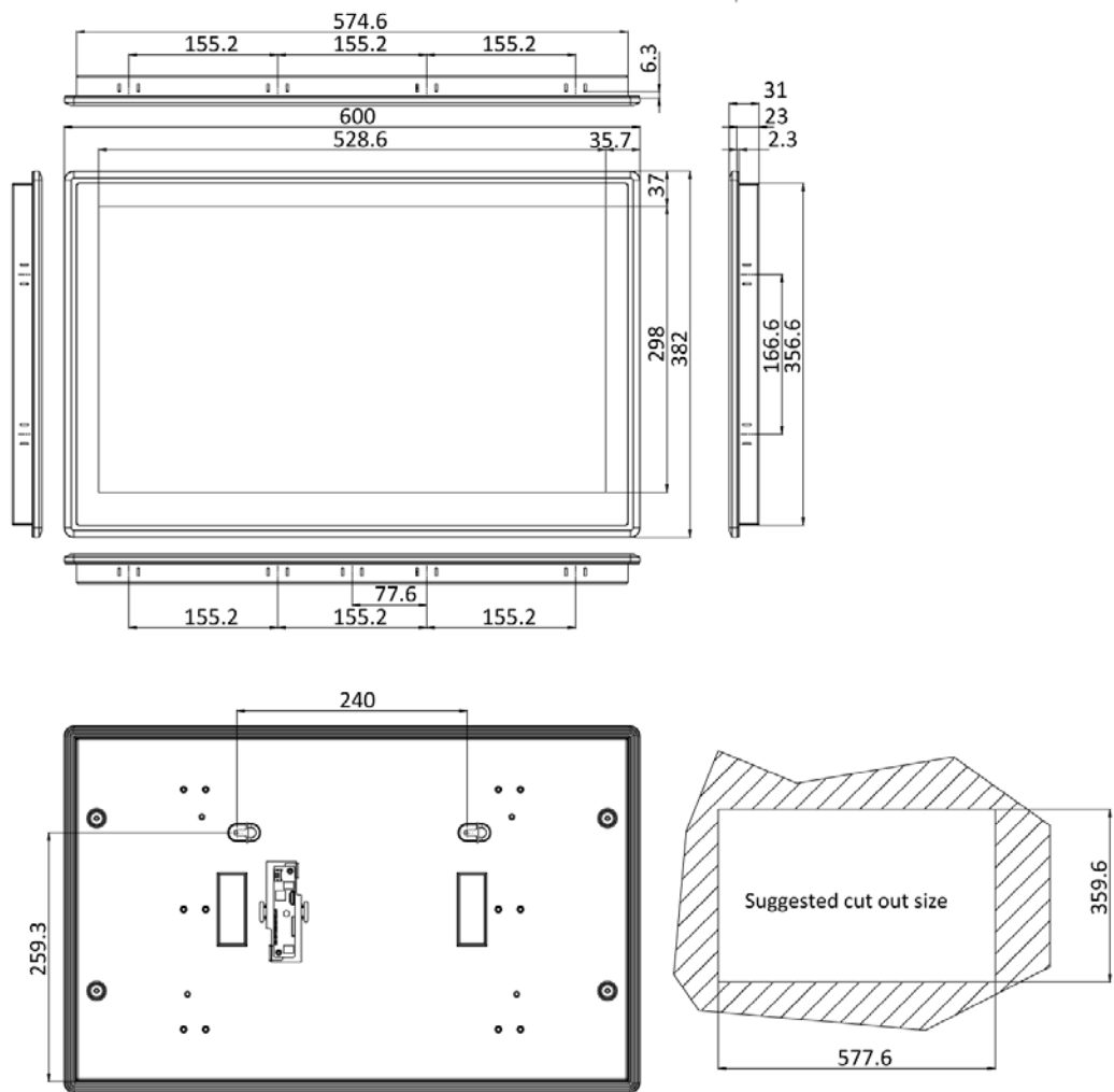
FLEX-PLKIT-FW24 Dimensions (mm)
