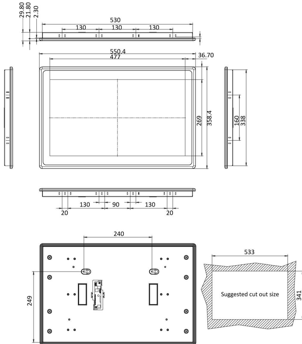
FLEX-PLKIT-FW22 Dimensions (mm)
