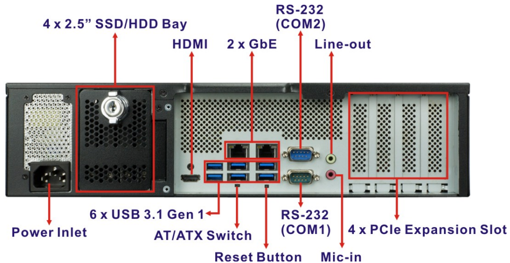
Figure 1-3: Rear Panel
